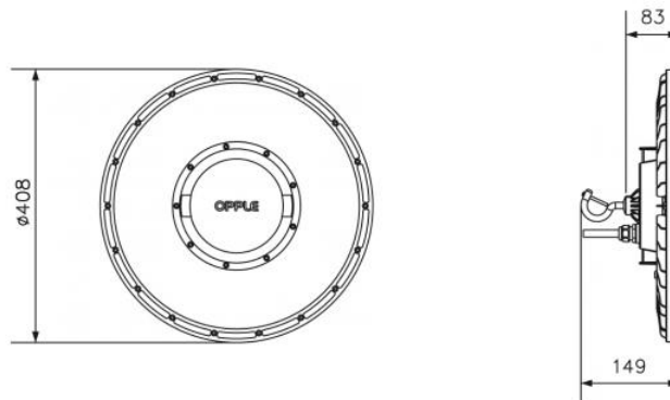
LEDHighbay-P4 155W & 230W
