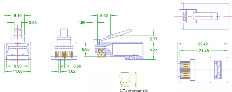
Connector
