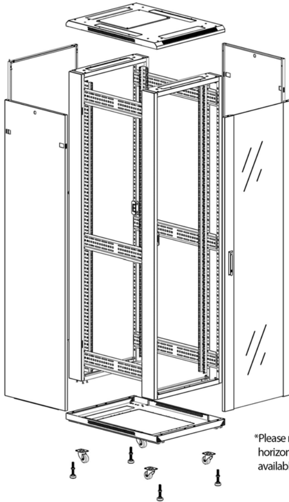
Removable side panel
