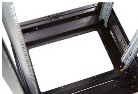
Large cut out in base for cable entry
