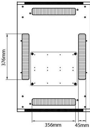
Roof
