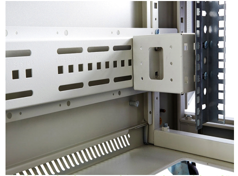
Full height front and rear adjustable 19" profiles
