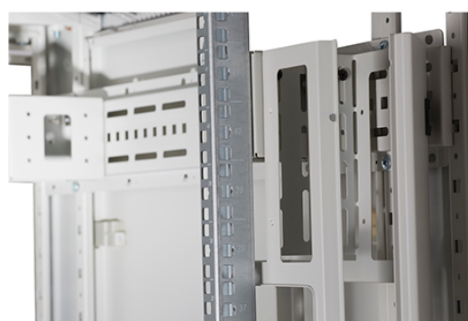
High-density vertical cable management
