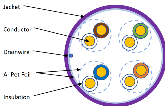
Cross-section diagram
