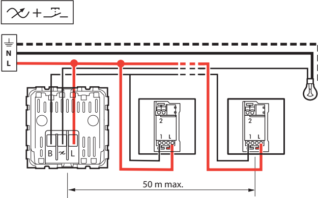
Wiring two-way switch
