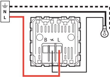
Wiring with Céliane pushbutton
