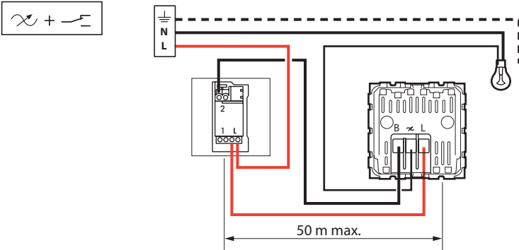
Wiring two-way switch
