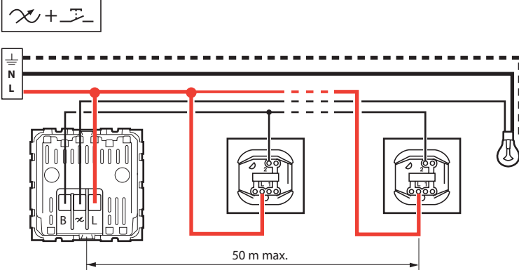
Wiring with Niloé pushbutton
