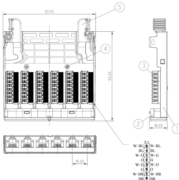
Product drawing
