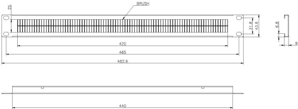
Product drawing (100-595)
