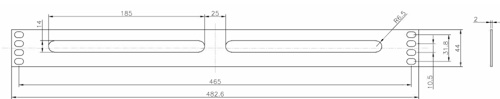
Product drawing (100-610)
