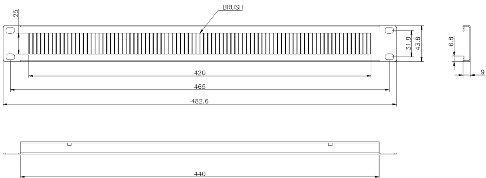
Product drawing (100-599)
