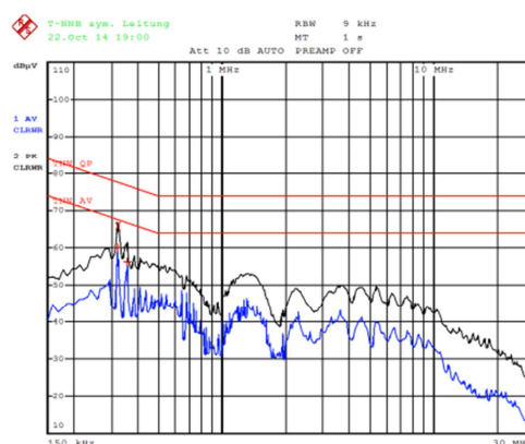
Interference Measurement DALI-line
