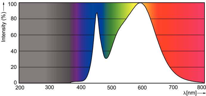
A60 /840 FR
