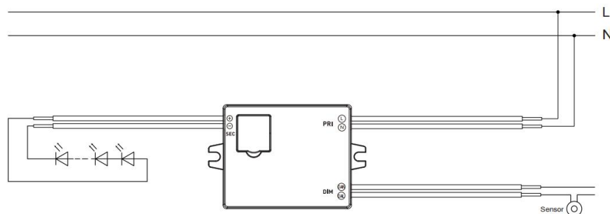
Wiring Diagram (Corridor Function)
