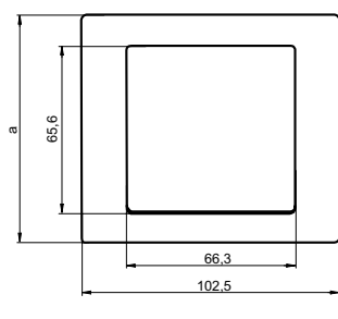
AQUADESIGN-Wippschalter
