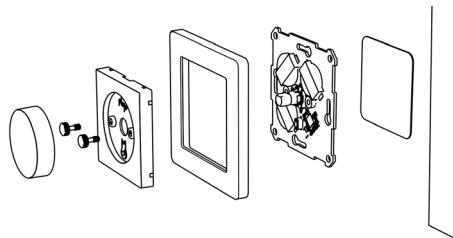
Mounting with accompanying tape on a wall.
