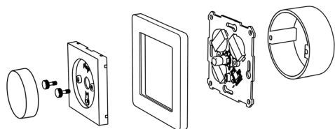
Mounting on the outside of an appliance box with screws.
