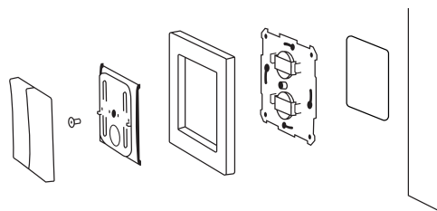
Mounting with accompanying tape on a wall.
