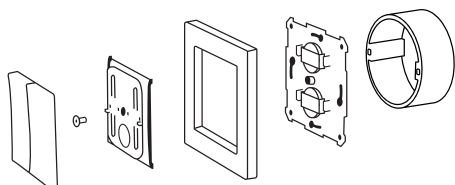
Mounting on the outside of an appliance box with screws.
